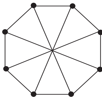
FIG. 2.1. The Möbius ladder ML_8 , also known as V_8 .
